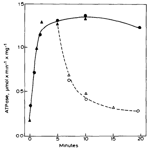
Fig.1. Reversible activation by glucose of the yeast plasma membrane ATPase. At time zero glucose was added to either commercial baker's yeast (triangles) or to the strain ATCC 42407 (circles) and samples were taken at the indicated times (closed symbols). After 5 min of incubation with glucose, part of the cells was washed by centrifugation in the cold and further incubated in the absence of glucose (open symbols). The ATPase activity of the total membrane fraction was determined at pH 5.7 with 2 mM ATP.
